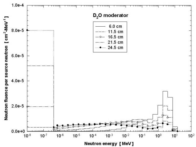
FIGURE 4. Neutron spectra, at 27 cm, produced by a ^{239}\text{PuBe} neutron source inserted at the center of a set of 6.0, 11.5, 16.5, 21.5 and 24.5-cm-radii \text{D}_2\text{O} moderator media.
