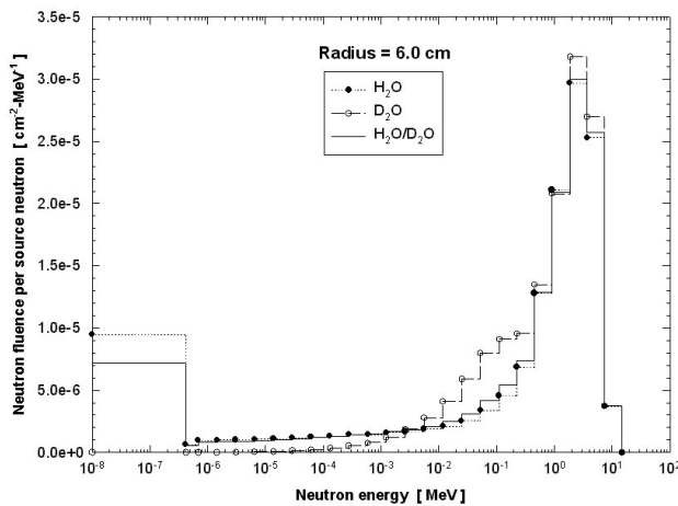
FIGURE 6. Neutron spectra, at 27 cm, produced by a 239 PuBe neutron source inserted at the center of 6.0-cm-radius moderator media (H 2 O, D 2 O and H 2 O/D 2 O).
