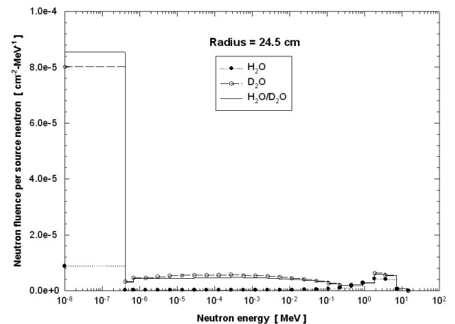
FIGURE 8. Neutron spectra, at 27 cm, produced by a 239 PuBe neutron source inserted at the center of 24.5-cm-radius moderator media (H 2 O, D 2 O and H 2 O/D 2 O).
