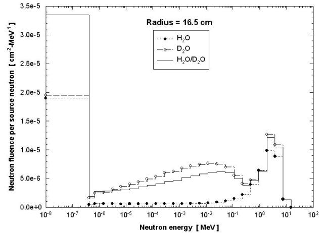
FIGURE 7. Neutron spectra, at 27 cm, produced by a 239 PuBe neutron source inserted at the center of 16.5-cm-radius moderator media (H 2 O, D 2 O and H 2 O/D 2 O).
