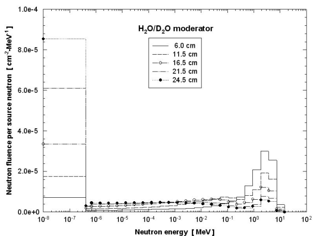
FIGURE 5. Neutron spectra, at 27 cm, produced by a ^{239}\text{PuBe} neutron source inserted at the center of a set of 6.0, 11.5, 16.5, 21.5 and 24.5-cm-radii \text{H}_2\text{O}/\text{D}_2\text{O} moderator media.
