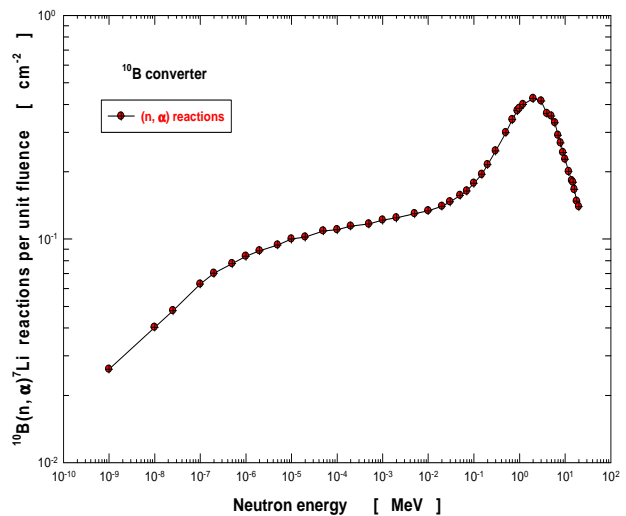
Figure 3. ^{10}\text{B} converter (n, \alpha) response.
