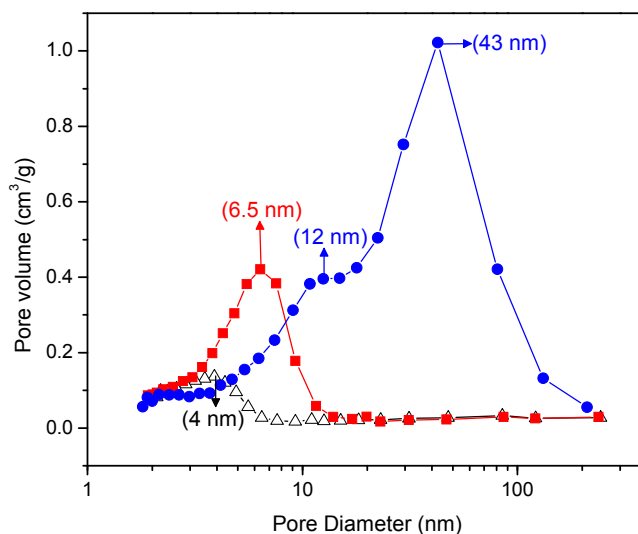
Figure 5. Pore size distribution of the Pt-TiO 2 prepared via incipient wetness impregnation; (●) mesoporous TiO 2 thermally treated at 550 °C (Guayaquil et al. [10] (sol-gel B), (■) mesoporous TiO 2 calcined at 450 °C (sol-gel A), (▲) Degussa P25 impregnated with 1.00 wt % Pt and calcined at 450 °C.
