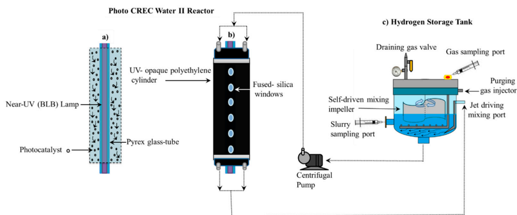
Figure 2. Schematic diagrams of the Photo-CREC Water II Reactor with a \text{H}_2 mixing/storage tank: (a) Longitudinal cross-section of the Photo-CREC Water II unit showing the downflow slurry circulation in the annular channel; (b) overall view of Photo-CREC Water II showing windows and recirculation pump and (c) hydrogen storage tank with its components. Adapted from [10].
