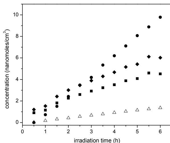
Figure 16. CO 2 increase with irradiation time for: (●) 2.50 wt % Pt-TiO 2 (sol-gel B), (■) 1.70 wt % Pt-TiO 2 (sol-gel A), (◆) 1.70 wt % Pt-TiO 2 (wetness impregnation) and (Δ) Degussa P25. Standard deviation for repeats is within \pm 5\% .
