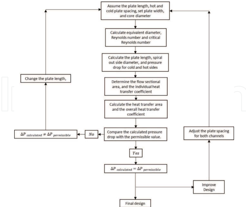
Figure 2. Flow chart to design the cross-flow spiral heat exchanger.
