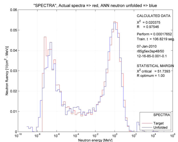
FIGURE 1. Neutron spectra unfolded with the optimized ANN.
