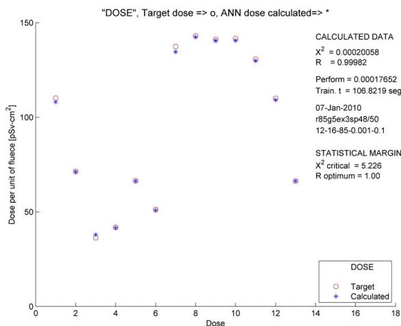
FIGURE 2. 13 equivalent doses calculated with the optimized ANN.
